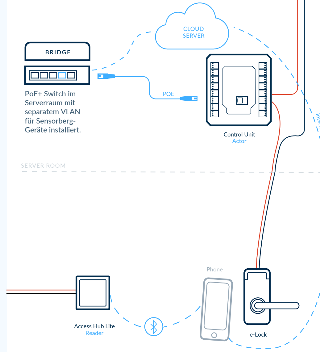
② Access Hub Lite Reader > Control Unit Actor
