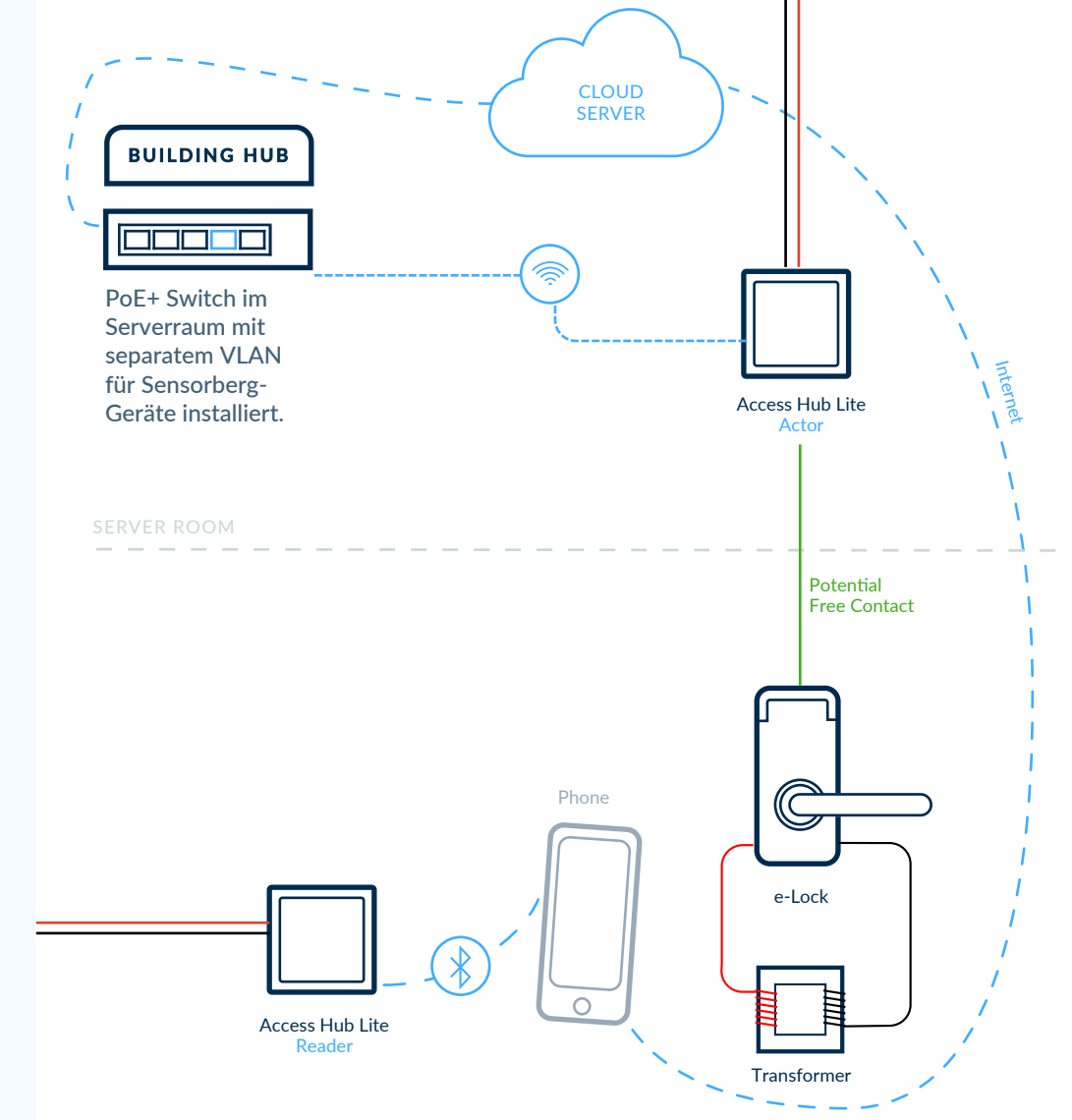
③ Access Hub Lite Reader > Access Hub Lite Actor
