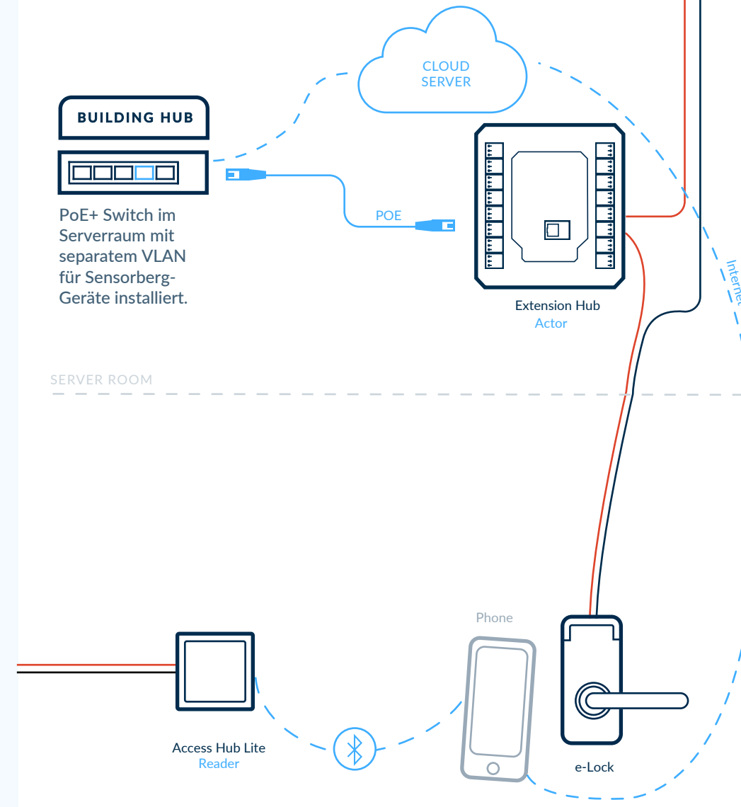
② Access Hub Lite Reader > Extension Hub Actor
